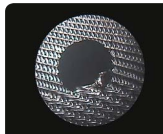
Metal filter with material covering at the end part of the filter before beading
